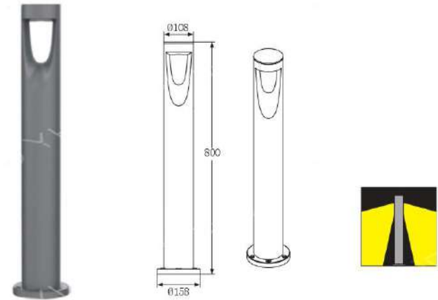
● P-023231-80 LED: LUMILEDS 12W
