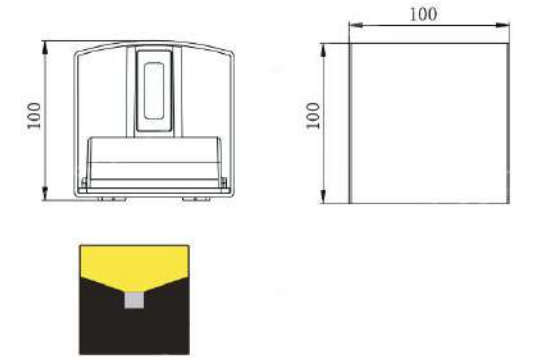
B-003061 LED: CREE-COB 3Wx2
