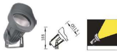
● G-013364DZ LED: CREE-COB 8W
